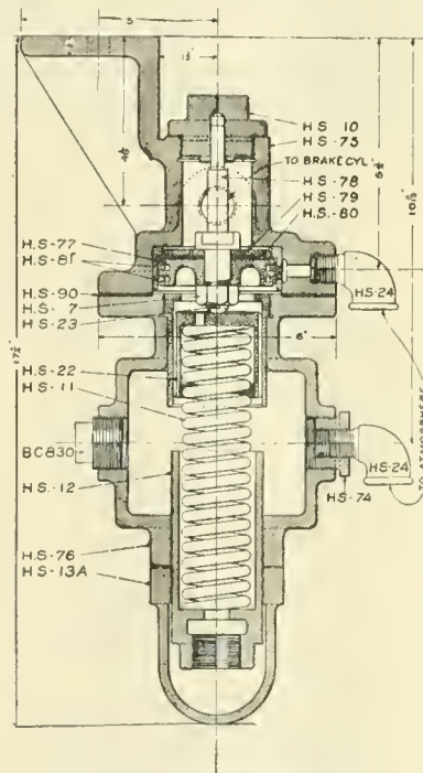
FIG. 1, COMPENSATING VALVE.
